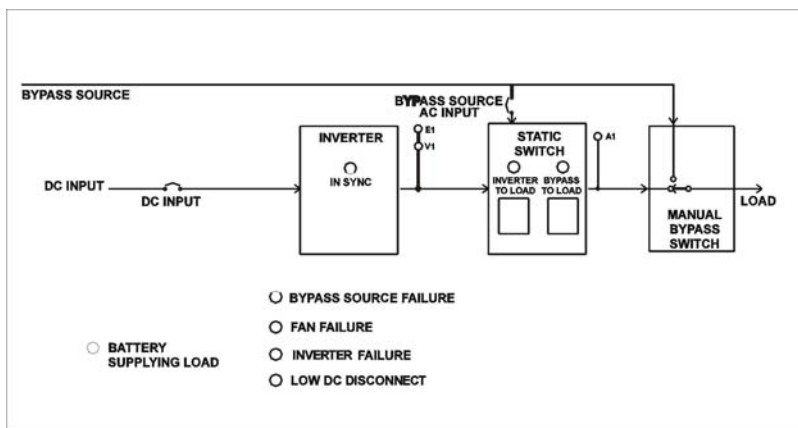
Figure 1.0 Mimic Panel/One-Line Diagram
